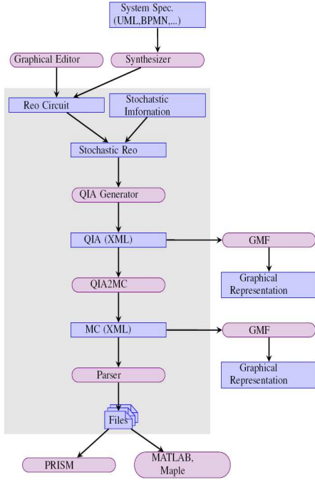
Figure 2: Architecture of Reo2MC
